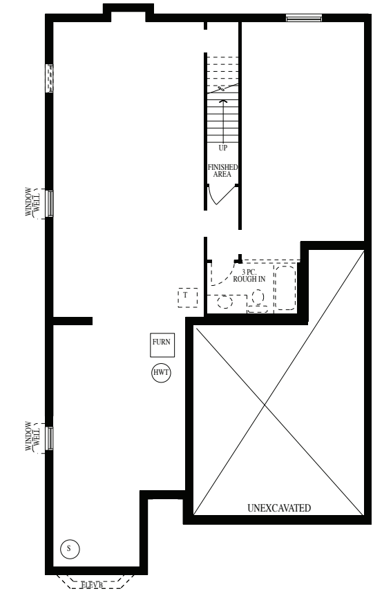
UNFINISHED BASEMENT ELEVATION 'A' & 'B'
