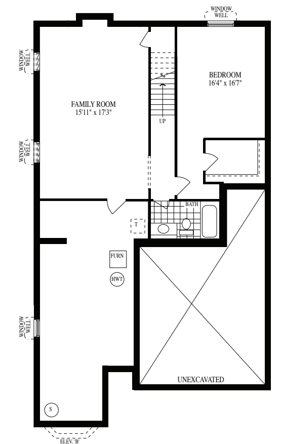
FINISHED BASEMENT ELEVATION 'A' & 'B'
