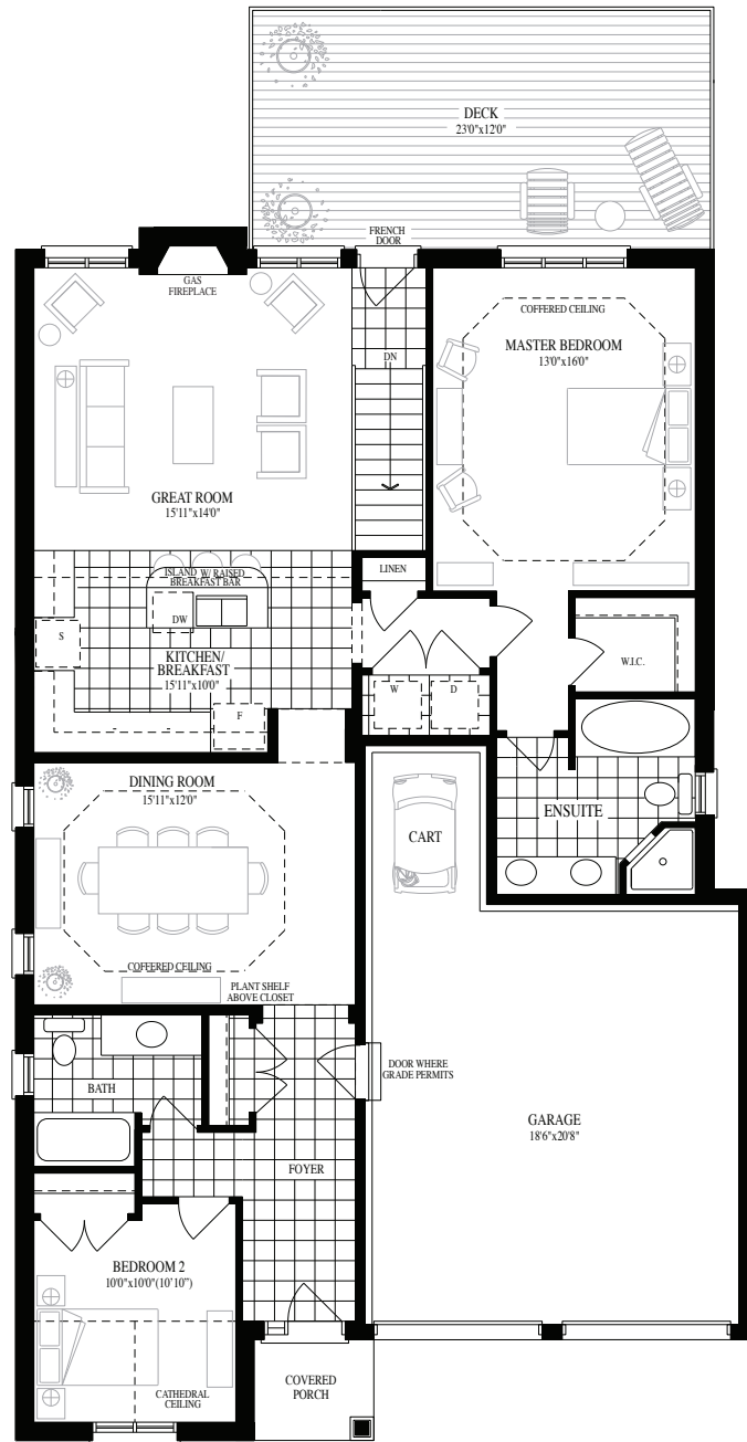
GROUND FLOOR
