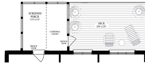
OPTIONAL SCREENED IN PORCH WITH DECK
