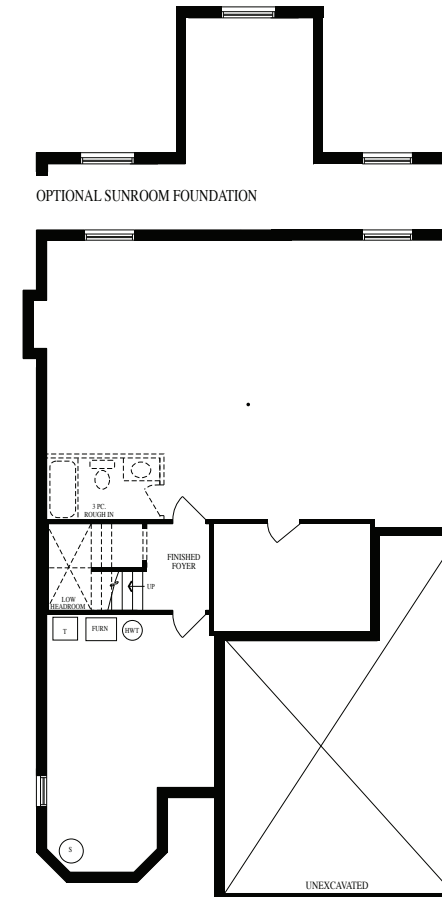
UNFINISHED BASEMENT ELEVATION 'A'
