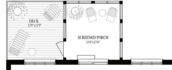
OPTIONAL SCREENED IN PORCH WITH DECK
